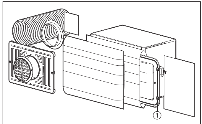
1 Service Kit 30260
