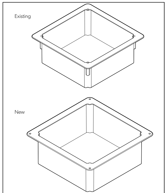
1 Existing 6 in. Clamp Garnish (GX) and New 6 in. Dometic Garnish (GDX)
