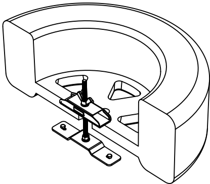
Spare Wheel Clamp Inverted
