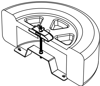
Spare Wheel Clamp Low Mount
