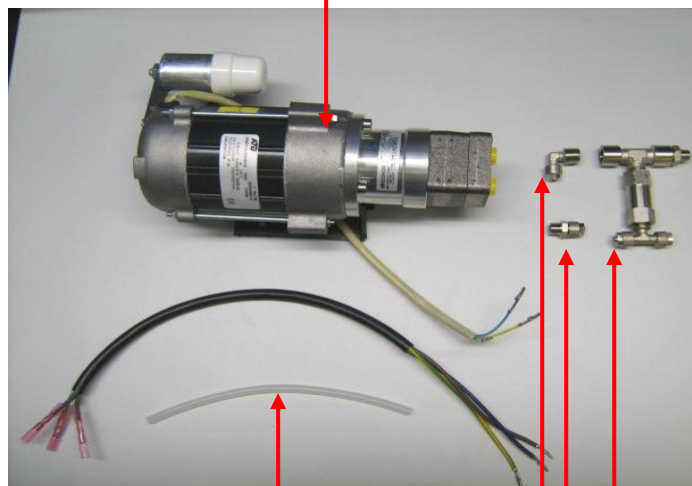
Accessory electric gear pump Art.Nr.: 4441600099
