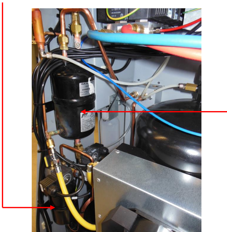
Oil separator Facelift Art.Nr.: 4440600124
