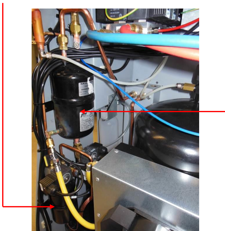
Oil separator Art.Nr.: 4440600124
