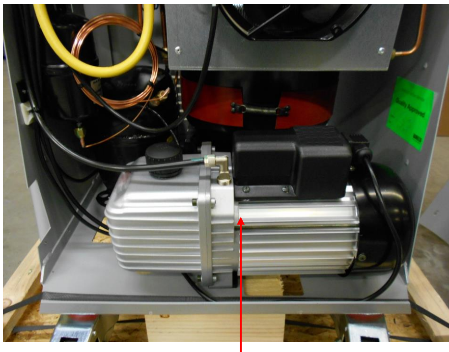
Vacuum pump ASC Art.Nr.: 4440600207
