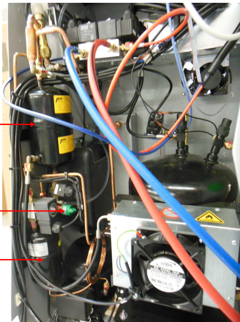
Pressure switch 16bar Art.Nr.: 4440600192
