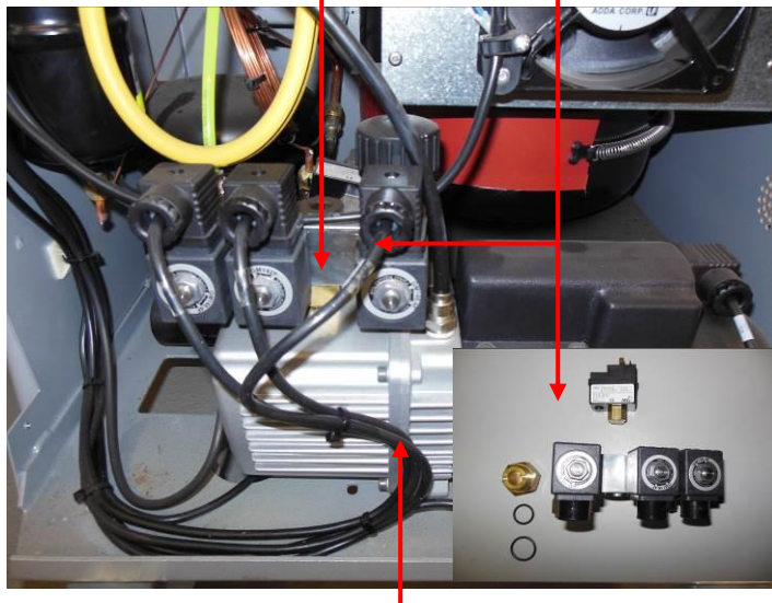
Vacuum pump ASC Art.Nr.: 4440600030
