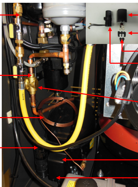
Copper pipe with sightglass Only RPA Sweden!!! Art.Nr.: 4440450078 Copper pipe RPA Standard accessory kit
