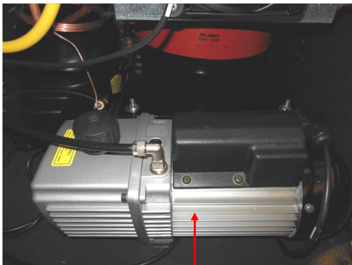
Vacuum pump ASC Art.Nr.: 4440600030
