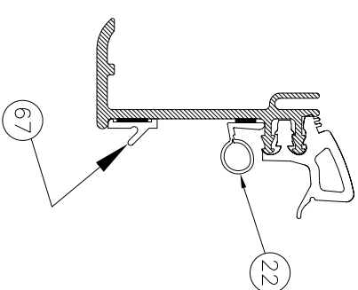
SECTION E-E SCALE: FULL
