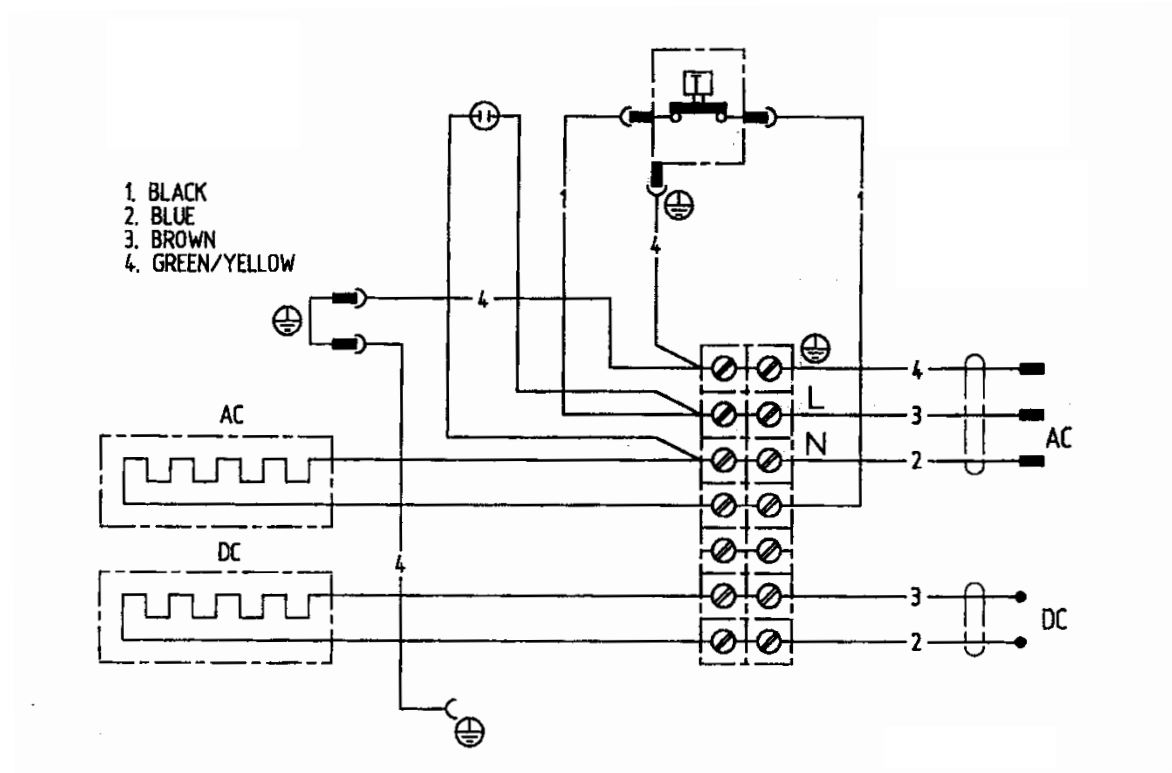
RC 3000 WIRING DIAGRAM
