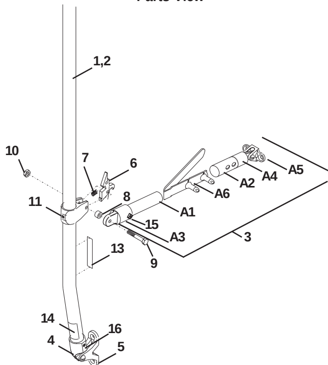
Parts View
