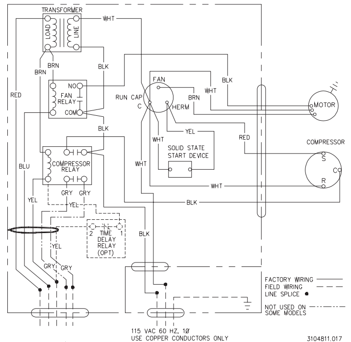
MODEL 39045.616
