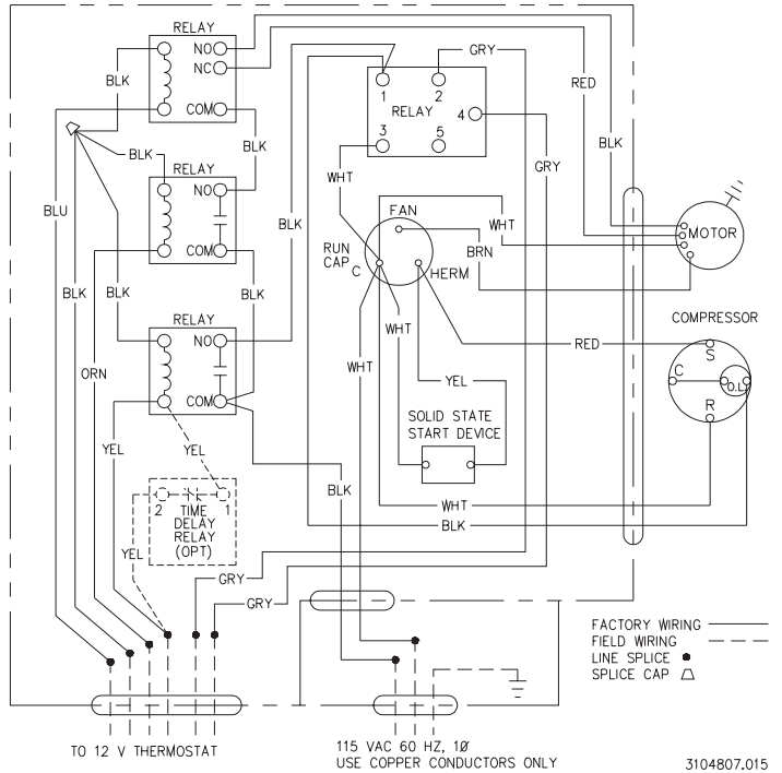
MODEL 39115.626
