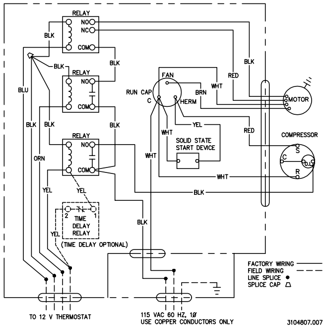
MODEL 39115.616
