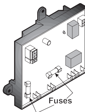
FIG. 2 Power Module 2931842.04
