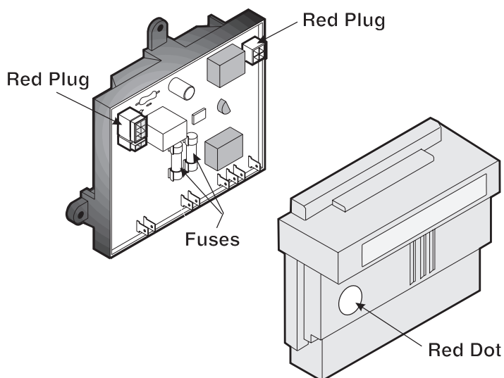
FIG. 2 Power Module 2931842.04
