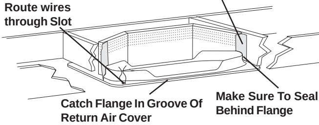
FIG. 22 Use Aluminum Foil Tape To Seal the Foam Divider To The Sides of 14-1/4" x 14-1/4" ( \pm 1/8 ") Ceiling Opening
