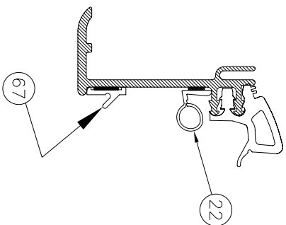
SECTION E—E SCALE: FULL
