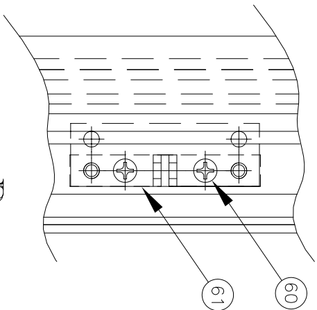
VIEW D SCALE: FULL
