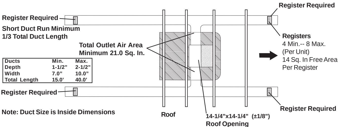
FIG. 7B Duct Size And Requirements For 3105007 And 3105935 Return Air Cover
