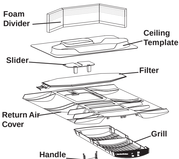
FIG. 27 Genesis Air Filtration System Return Air Kit
